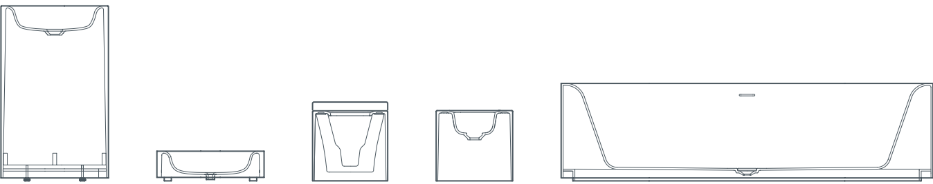
moon washbasin freestanding 55x45x90 cm moon washbasin countertop 55x45x16 cm moon toilet wall hung 56x39x36 cm moon bidet wall hung 56x39x36 cm moon bath freestanding 190x90x50 cm
