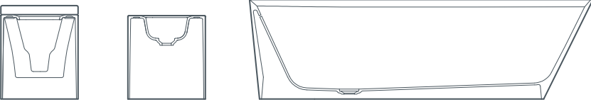
pearl toilet floor mounted 56x39x42 cm pearl bidet floor mounted 56x39x42 cm pearl bath oval freestanding 172x81x50 cm
