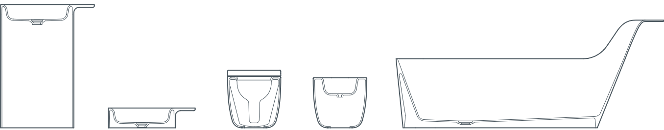
pride washbasin freestanding 67 x 43 x 90 cm pride washbasin countertop 67 x 40 x 15 cm pride toilet wall hung 58 x 39 x 37 cm pride bidet wall hung 58 x 39 x 37 cm pride bath freestanding 192 x 85 x 78 / 50 cm
