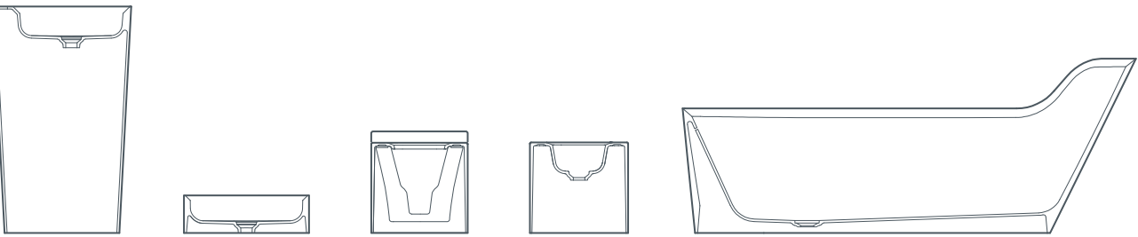
pearl washbasin freestanding 55x40x90 cm pearl washbasin countertop 50x40x15 cm pearl toilet wall hung 56x39x36 cm pearl bidet wall hung 56x39x36 cm pearl bath freestanding 182x81x70/50 cm
